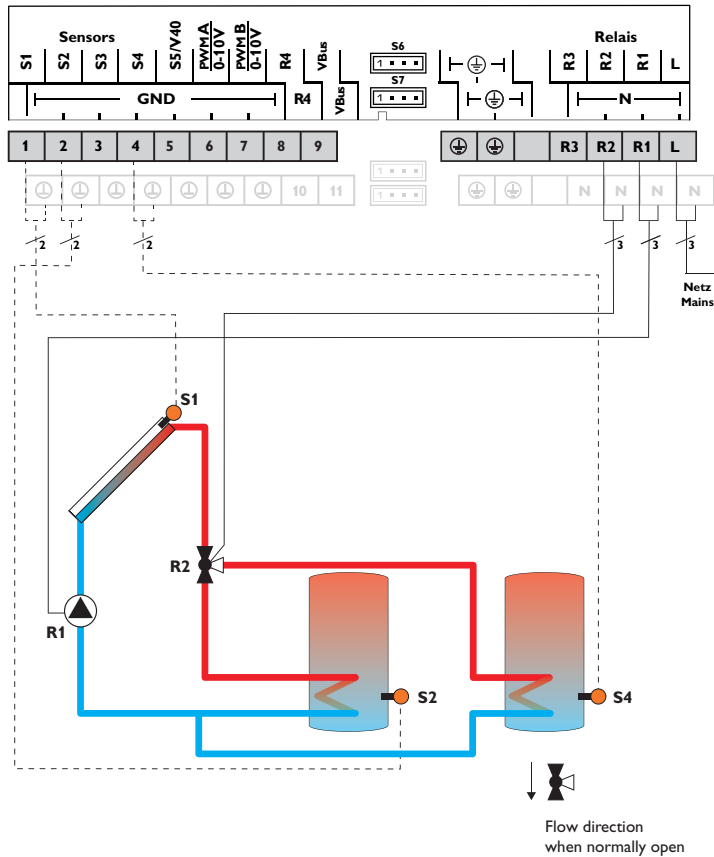
Hydraulic variant 1
